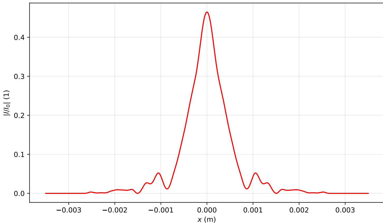
Intensity profile I(x, y = 0, z = 2.149)/I_0 , P_{in}=5.0P_{cr} , artificial time
